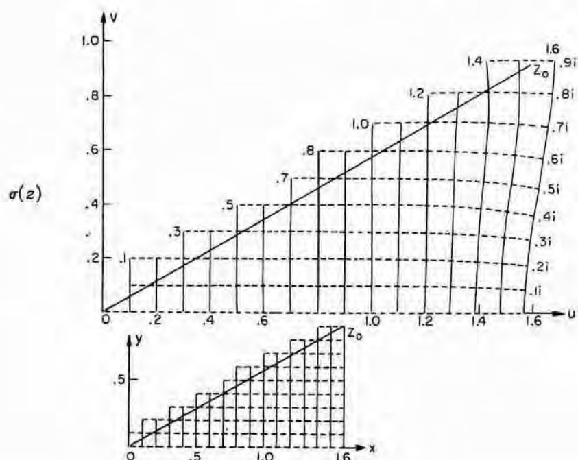
FIGURE 18.12
