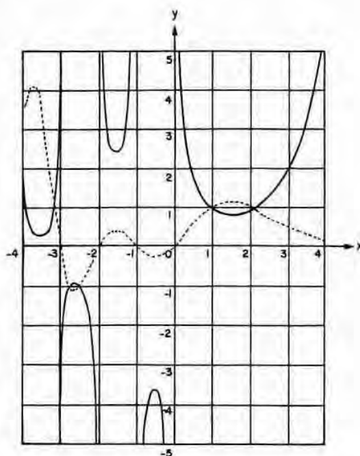
FIGURE 6.1. Gamma function. *
