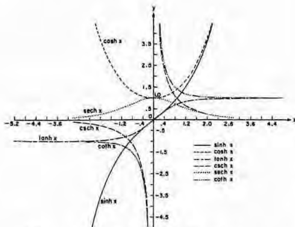
FIGURE 4.6. Hyperbolic functions.
