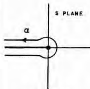
FIGURE 19.1 -\pi < \arg z < \pi
