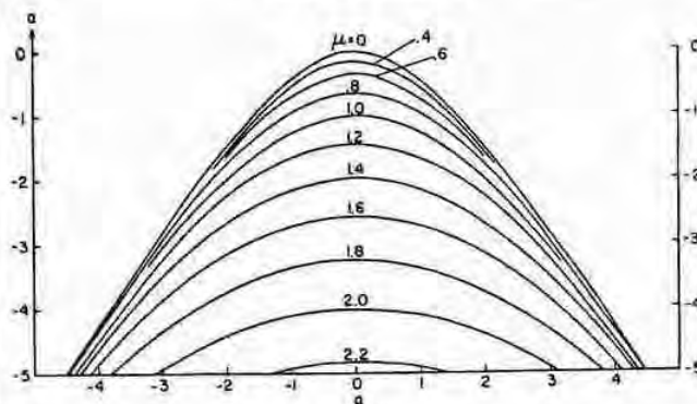
FIGURE 20.7. Characteristic Exponent in First Unstable Region. Differential equation: y'' + (a - 2q \cos 2x)y = 0 . The Floquet solution y = e^{i\nu}P(x) , where P(x) is a periodic function of period \pi . In the first unstable region, \nu = i\mu ; \mu is given for a \geq -5 . (Constructed at NBS.)
