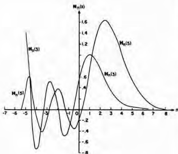
FIGURE 12.3. Struve functions.
