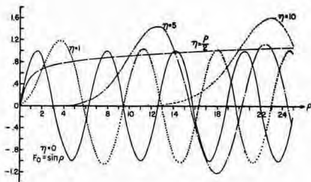
FIGURE 14.3. F_0(\eta, \rho) .
