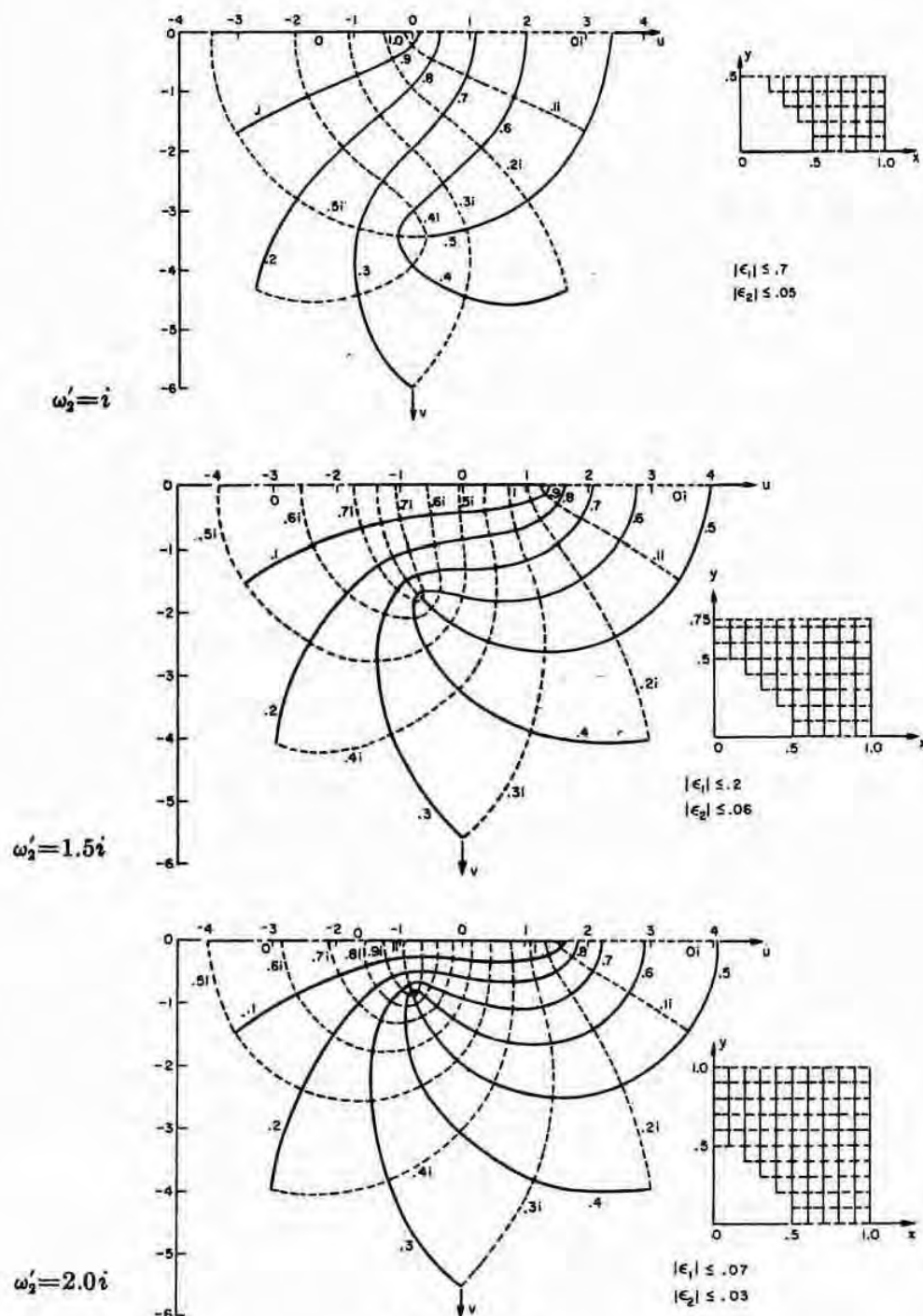
FIGURE 18.6
