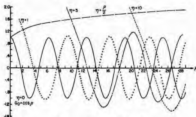
FIGURE 14.5. G_0(\eta, \rho) .
