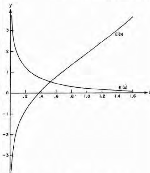
FIGURE 5.1. y = \operatorname{Ei}(x) and y = E_1(x) .
