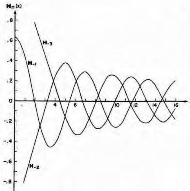
FIGURE 12.2. Struve functions.
