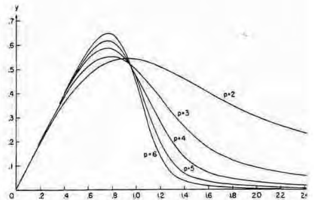
FIGURE 7.2. y = e^{-z^2} \int_0^z e^{t^2} dt . p=2(1)6
