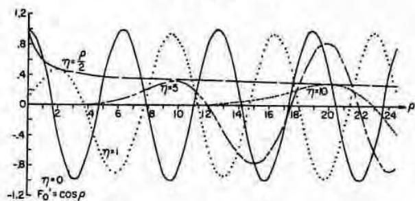
FIGURE 14.4. F'_0(\eta, \rho) .
