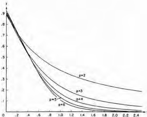
FIGURE 7.1. y = e^{z^2} \int_z^\infty e^{-t^2} dt . p=2(1)6
