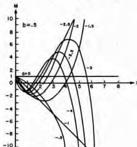
FIGURE 13.4. M(a, .5, x) .
