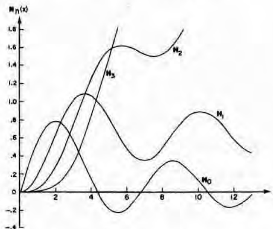
FIGURE 12.1. Struve functions.
