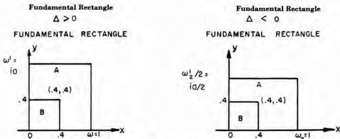
FIGURE 18.4
