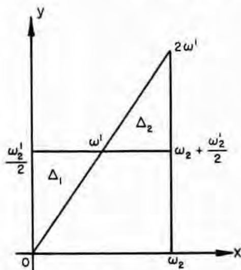
FIGURE 18.3
