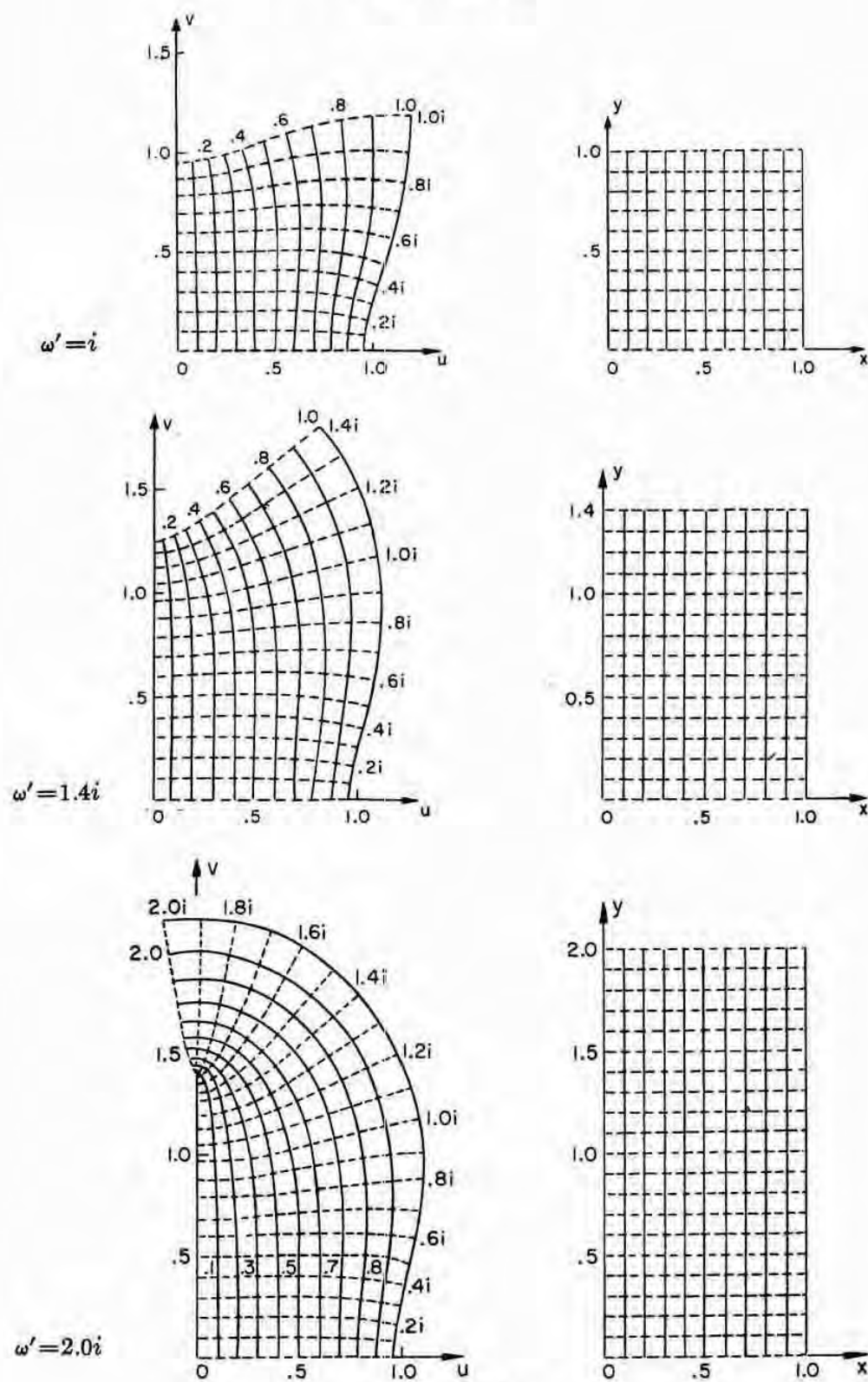
FIGURE 18.9
