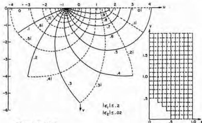
FIGURE 18.5
