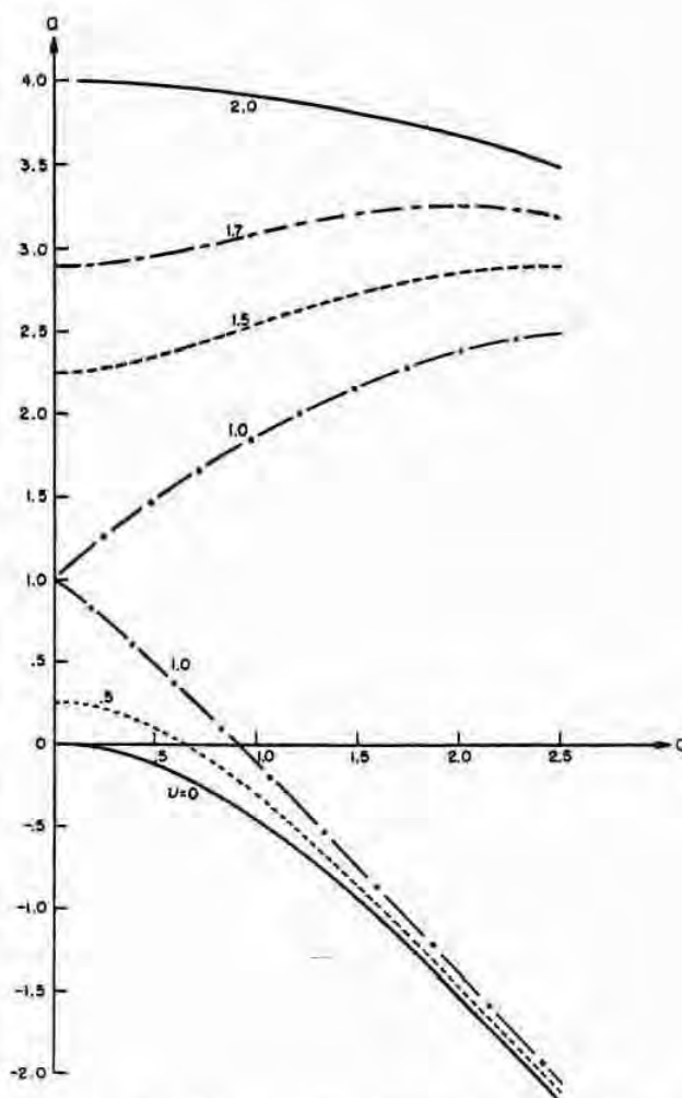
FIGURE 20.6. Characteristic Exponent—First Two Stable Regions y = e^{i\nu}P(x) where P(x) is a periodic function of period \pi .
