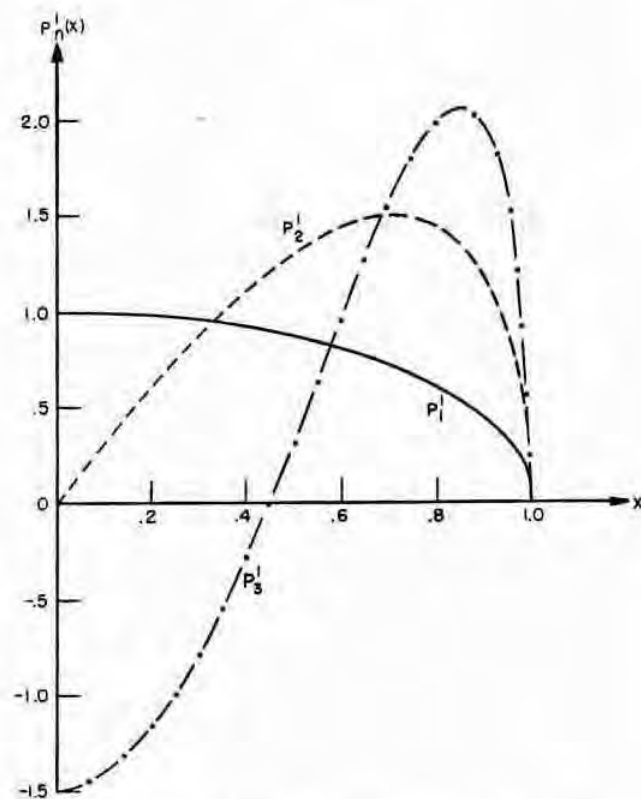
FIGURE 8.2. P_n^l(x) . n=1(1)3, x \leq 1 .
