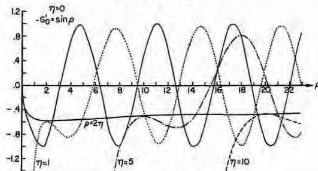
FIGURE 14.6. G'_0(\eta, \rho) .
