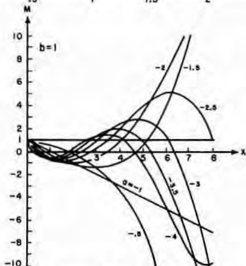
FIGURE 13.3. M(a, 1, x) .
