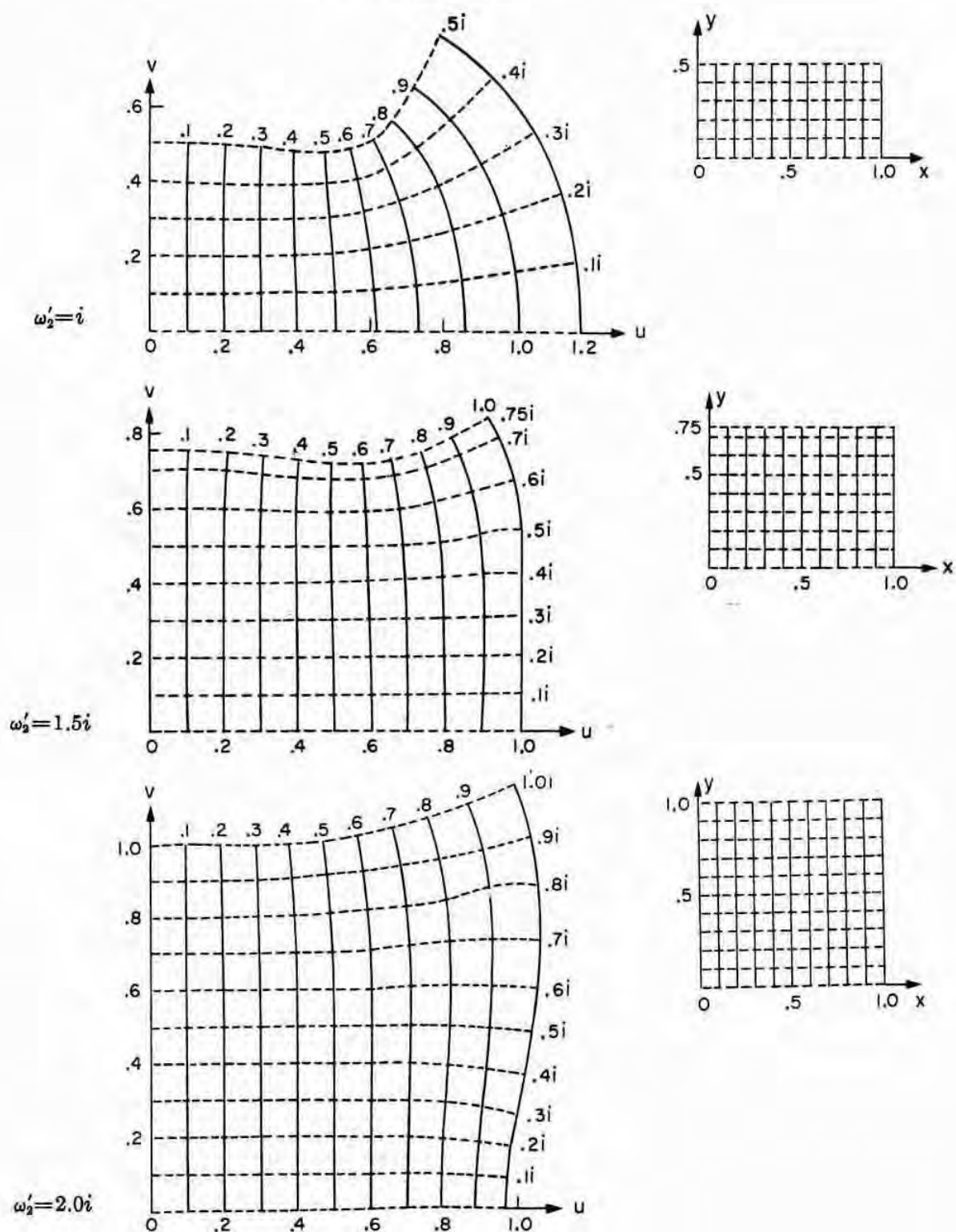
FIGURE 18.10
