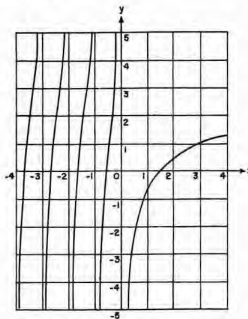
FIGURE 6.2. Psi function.
